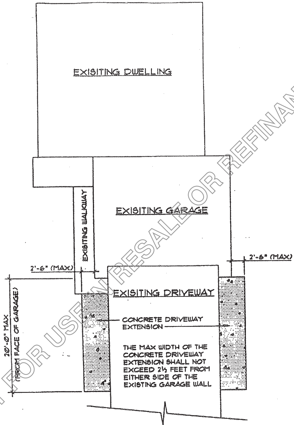
EXHIBIT N Concrete Driveway Extension Standard
